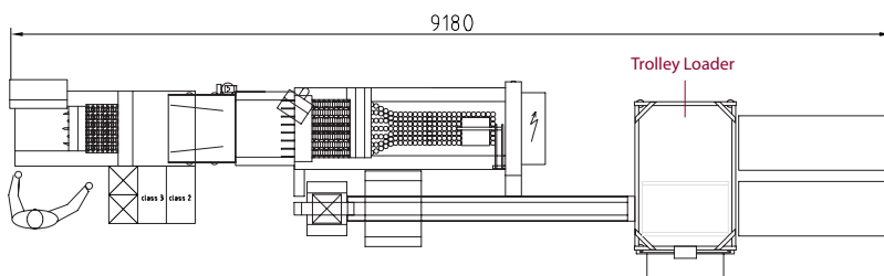
Ovograder 30 with Ovoset Pro & Trolleyloader
