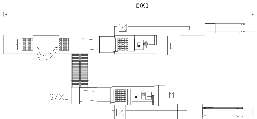
Ovograder 30 with integrated candling unit, two Smartpack units and PS4 tray stackers
